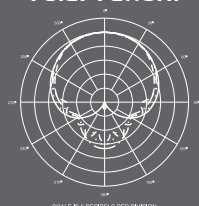
Polar Pattern
