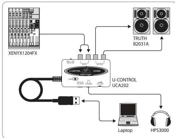
Fig. 4.1: Common version with the UCA202
