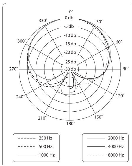
Polar Pattern
