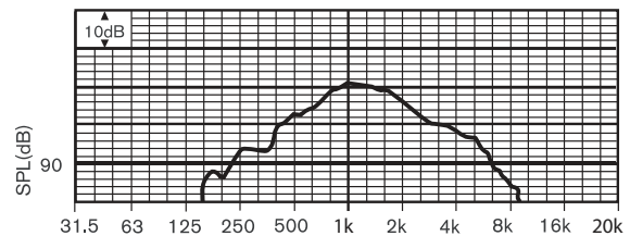
Frequency response
