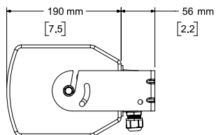
Right View DIMENSIONS APPLY TO BOTH SIDES
