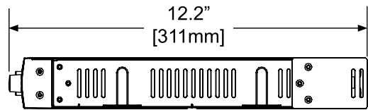
Right View
