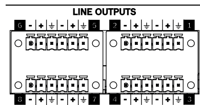
Figure 5.2: Analog output connections
