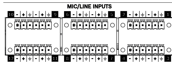
Figure 5.1: Analog input connections
