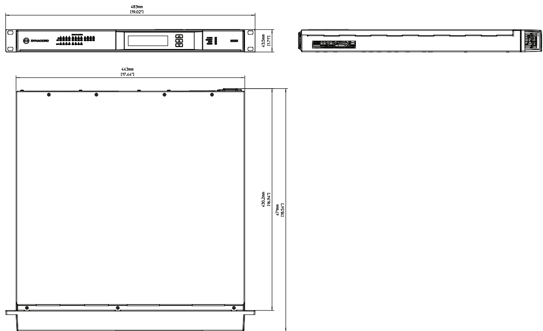
Figure 7.1: Dimensions: MXE5
