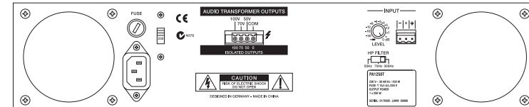
PA1250T rear view
