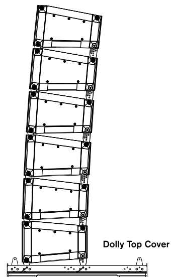
Dolly Top ground-stacking
