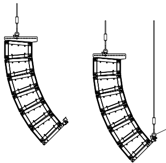
X12TC-GRID WITH PULL-BACK TO VENUE
