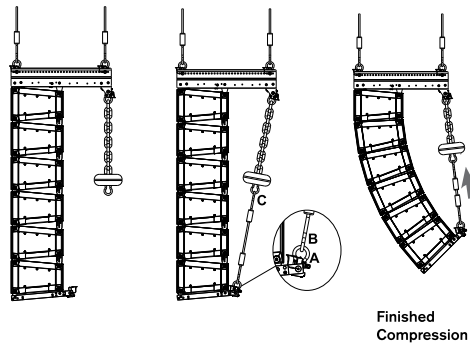
X12TE-GRID X12PU-BGK TO PULL-UP TO GRID
