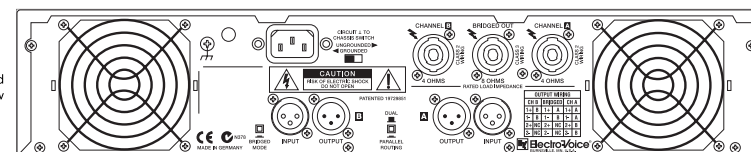
CP3000S and CP4000S rear view
