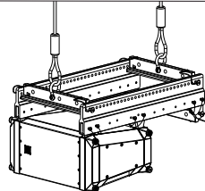
X12TC-GRID PULL-UP KIT
