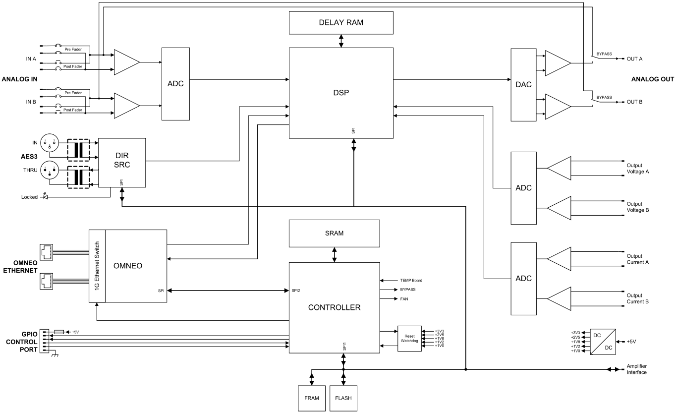
Circuit diagram
