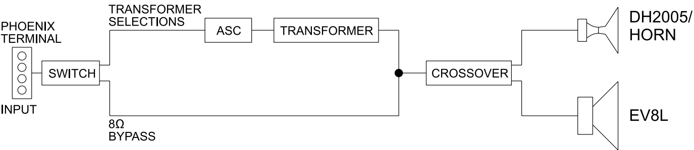
Fig. 2: ZX1i (With transformer)
