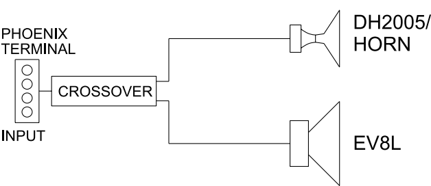
Fig. 1: ZX1i (Non-Transformer) and ZX1i (With transformer) in 8 ohm mode
