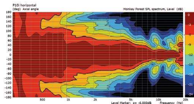
Horizontal directivity
