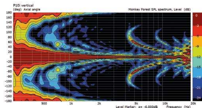
Vertical directivity
