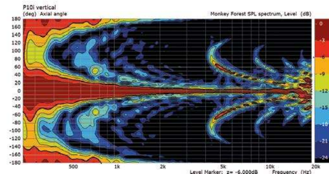
Vertical directivity
