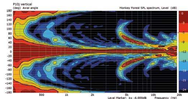
Vertical directivity
