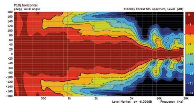
Horizontal directivity
