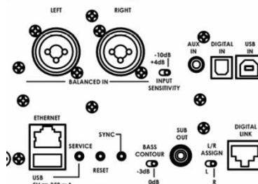
Secondary Speaker – Back Panel Connections
