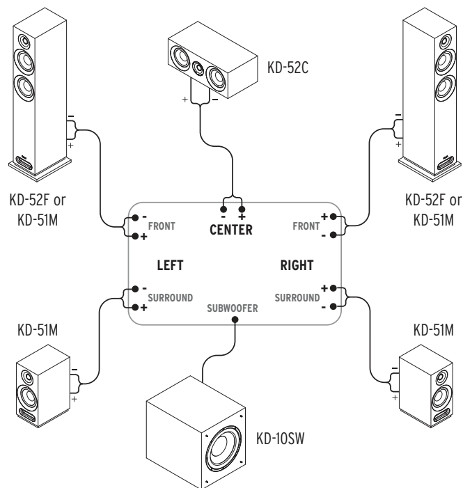
FIGURE 4 CONNECTING TO AV RECEIVER
