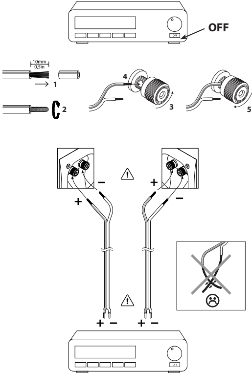
FIGURE 3 CONNECTING TO AV RECEIVER
