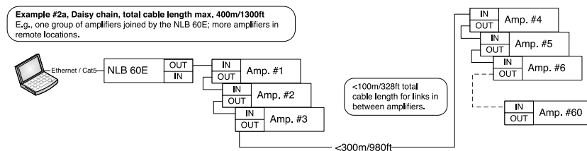
Figure 5.7.5c: NomadLink closed loop daisy chain configuration
