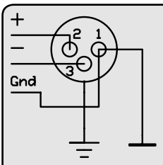
Figure 5.4.1c: Balanced XLR wiring schematic
