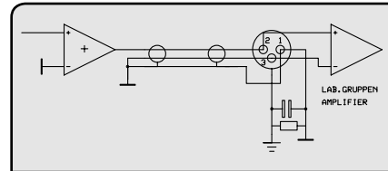
Figure 5.4.2: Unbalanced XLR wiring schematic
