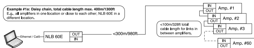
Figure 5.7.5a: NomadLink daisy chain configuration
