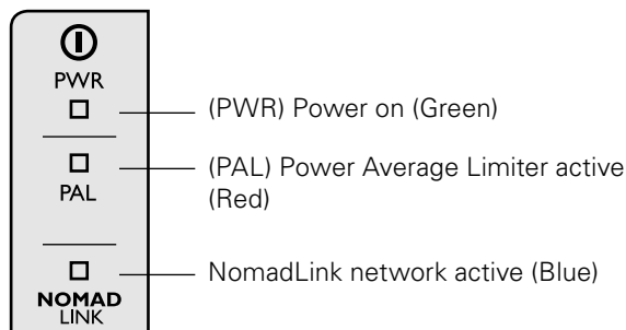
Figure 4.1.2b: Front panel global LED field
