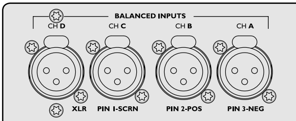
Figure 5.4.1a: Audio inputs - four-channel models
