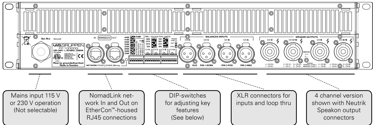
Figure 4.2: Two- and four-channel speaker output connector options (not applicable to all models)
