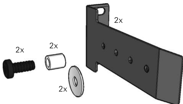
Figure 3.2a: Rear support mounting hardware
