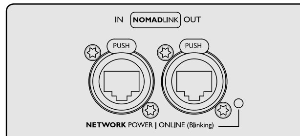
Figure 5.7.1: NomadLink Network RJ45 connectors
