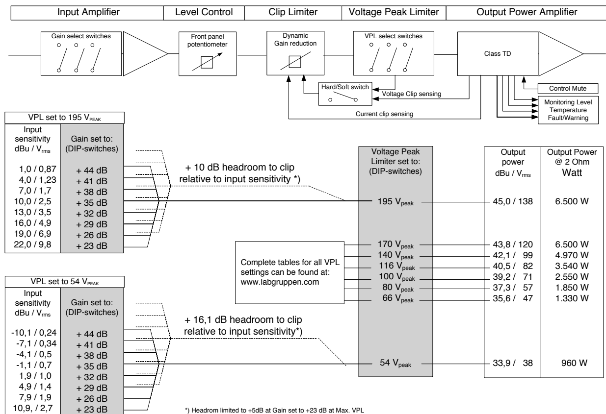
Figure 5.3.2: FP 13000 VPL and GAIN settings
