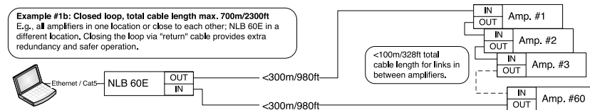
Figure 5.7.5b: NomadLink closed loop configuration
