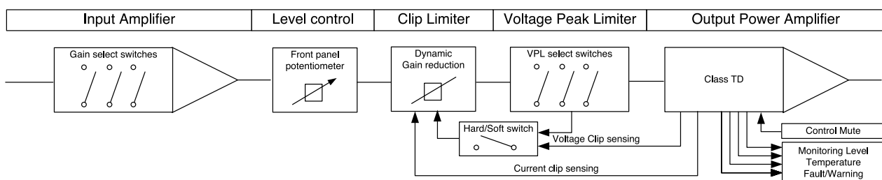
Figure 5.3.1: FP+ Series signal flow diagram
