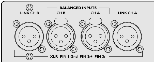
Figure 5.4.1a: Audio inputs and loop-thru
