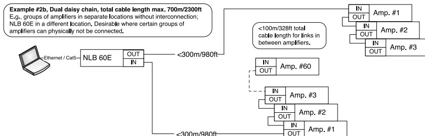
Figure 5.7.5d: NomadLink dual daisy chain closed loop configuration
