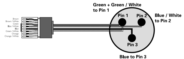
Figure 5.7.2: NomadLink RJ45 to XLR wiring schematic
