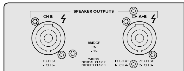
Figure 5.4.3a: Speakon outputs - two-channel
