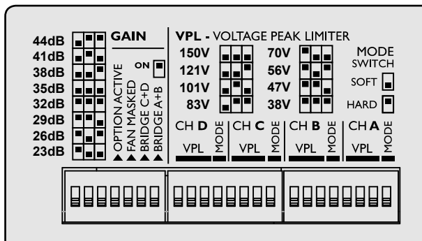
Figure 4.2.2a: Rear panel DIP-switch field
