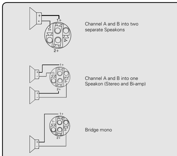
Figure 5.4.3c: Speakon wiring schematic
