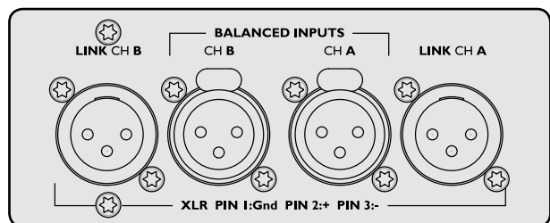
Audio inputs and loop-thru connectors - two-channel models
