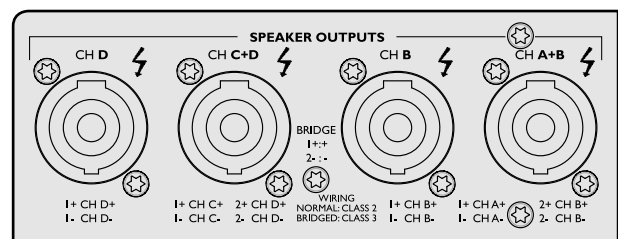
Figure 5.4.3b: Speakon outputs - four-channel
