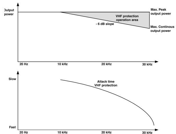
Figure 5.5.3: VHF protection attack time vs output power/frequency
