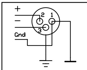
Figure 8.9: IEC268 XLR Wiring and Pin Out
