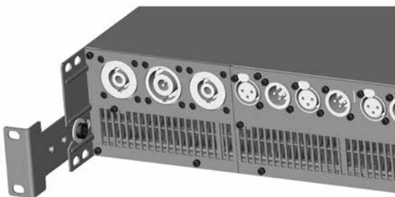
Fig 3.2: Rear support bracket mounted for fixed installation and bracket pointing forward
