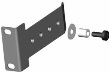
Fig 3.1: Rear support bracket with mounting hardware
