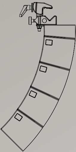
CURV 500 TMB Clamp for Truss
