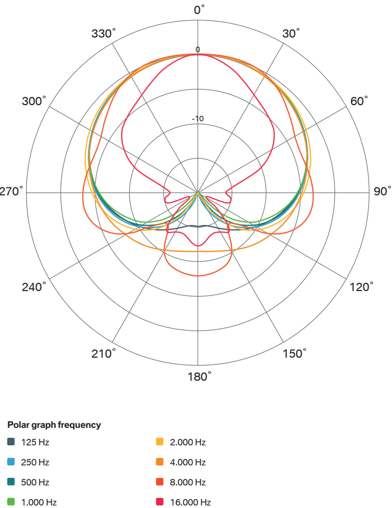
Figure 9.2 - Polar graph of the LCT 240 PRO
