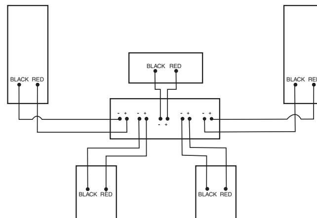
Figure 4- Connecting Speakers to Amplifier or Receiver
