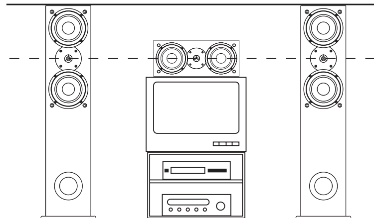
Figure 3- Proper Placement of Center Channel Speaker
