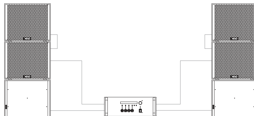
NXAMP4X4 powering 3 X MSUB18 (one in cardio mode) per side
