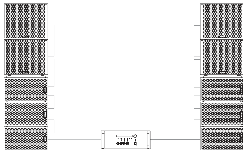
NXAMP4X4 powering 3 X GEO M12 and 2 X MSUB18 per side
