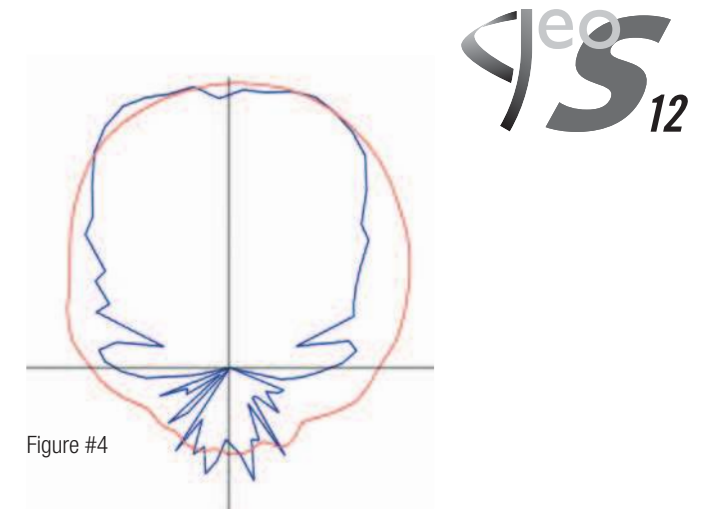
Figure #1: GEO S12 Hyperbolic Reflective Wavesource Figure #2: GEO S1210 Figure #3: GEO S1230 Figure #4: Relative coverage characteristics, at 4kHz, between arrayed S12 Series "hard" (coupled) coverage patterns (seen in blue) and "soft" (non-coupled) coverage (seen in red).
