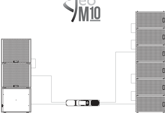
NXAMP4X2 Mk2 powering 3 X MSUB15 (one in cardio mode) and 6 X GEO M10
