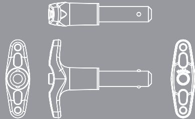
Quick release pin for GEOS8/GEOS12/RS15 Part Number #VXT-BL820
