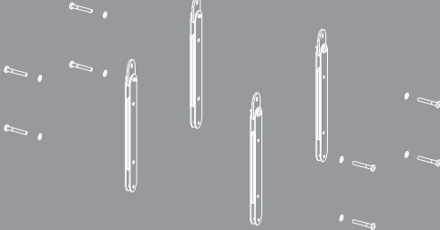
Installation Rigging Bars for RS15 Part Number #RSI-INSP15
