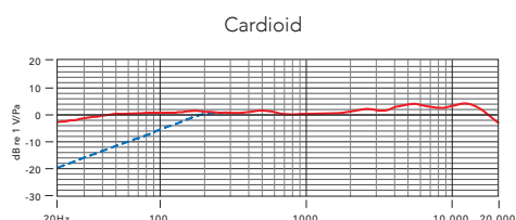
Cardioid
