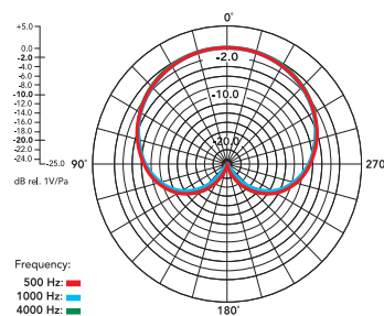
Cardioid capsule
