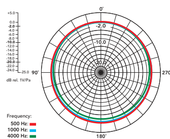
Omni capsule
