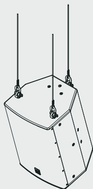
Hanged using the M8 screw threads.
