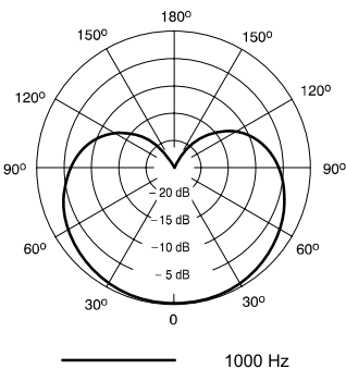
Polar Pattern
