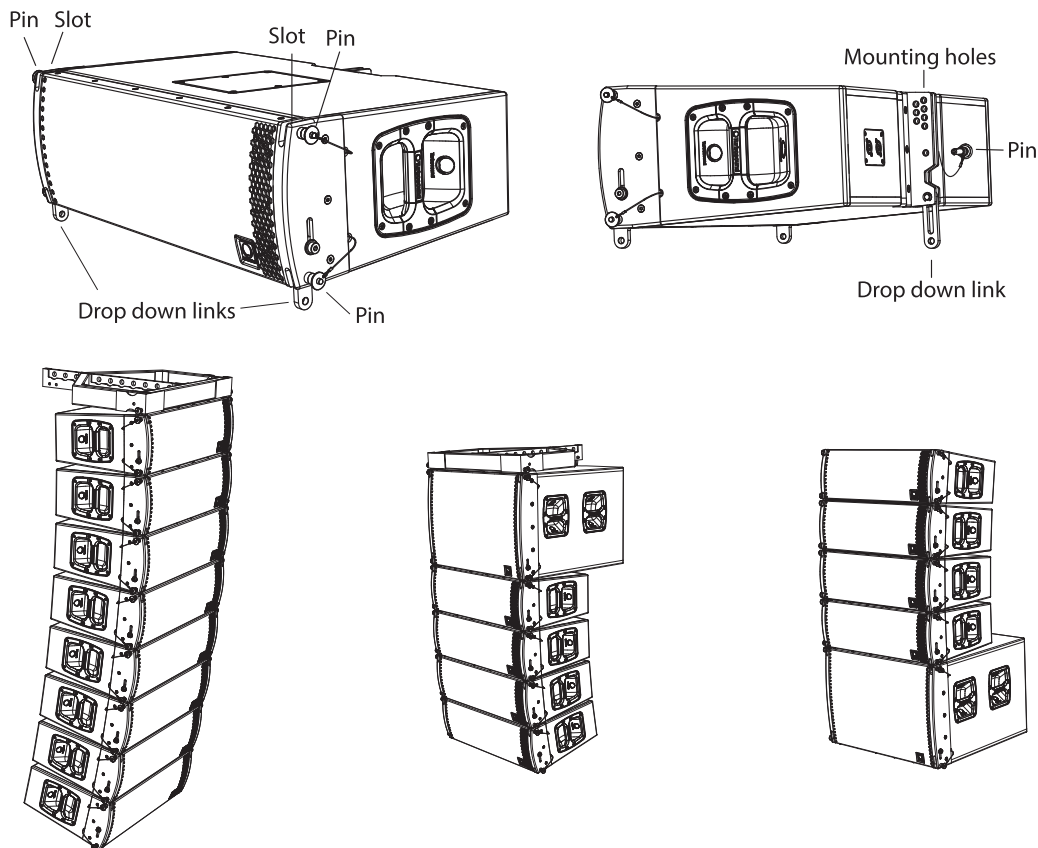
An array of 8 TLX84 cabinets attached to a TLX84-FLB flybar
