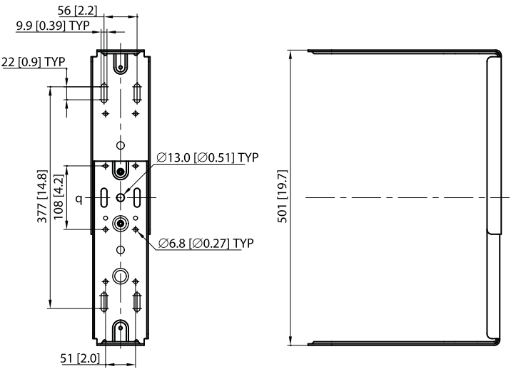
HORIZONTAL MOUNTING
