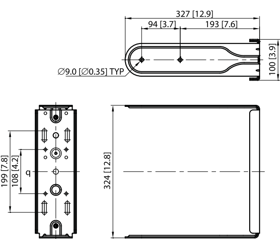
VERTICAL MOUNTING
